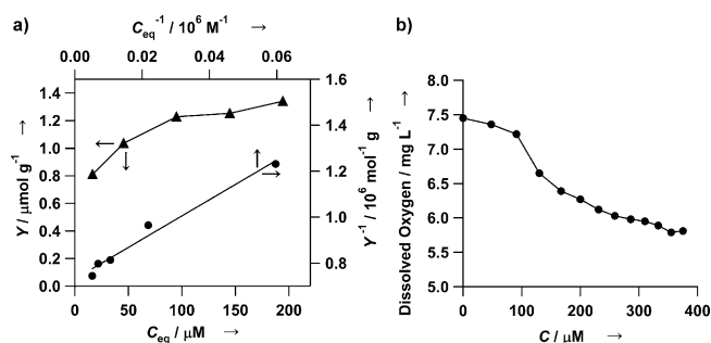
Figure 1. a) Cu adsorption isotherm on ms -BiVO 4 from the Cu(acac) 2 solution at 298 K and the Langmuir plot. b) Change in the amount of dissolved O 2 in an aqueous suspension of BiVO 4 with the addition of Cu(acac) 2 in a closed system.
